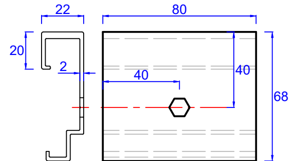
Locking bolt S-LK0480250.A2
