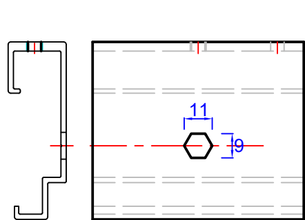
Adjusting bolt S-SKT0600300.A4.12
